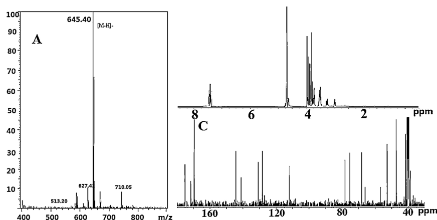
Fig. 1. Spectra of (Gly-Gly) 3 -Me and O,N -CMCS-(Gly-Gly) 3 -Me. (A) MS spectra of (Gly-Gly) 3 -Me; (B) 1 H NMR spectra of O,N -CMCS-(Gly-Gly) 3 -Me in D 2 O; (C) 13 C NMR spectra of O,N -CMCS-(Gly-Gly) 3 -Me in d 6 -DMSO.
